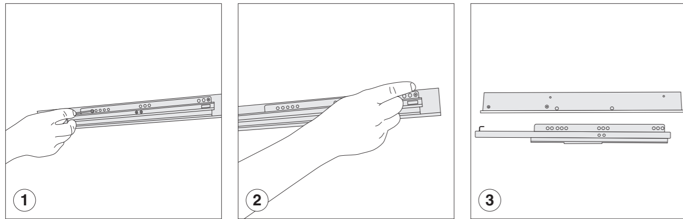
Svitare dalle piastre le guide scorrevoli (fig. 1-2-3). Unscrew the sliding guides from the plates (fig. 1-2-3).
