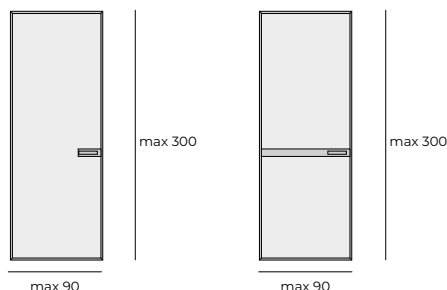
Anta scorrevole Sliding door
